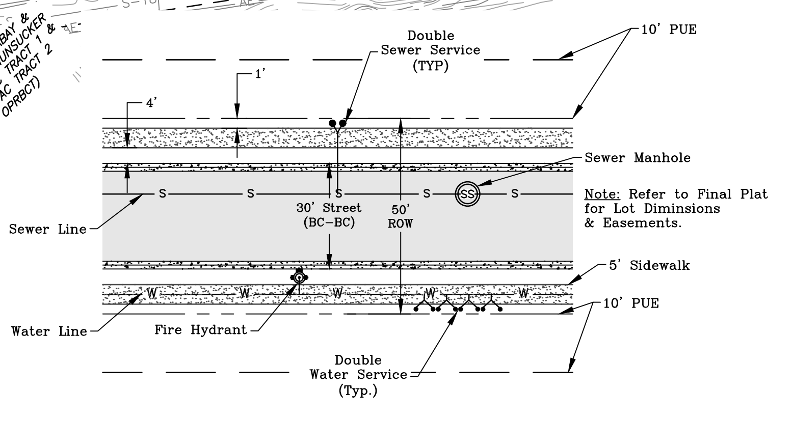
Typical Street & Utility Layout: N.T.S.
